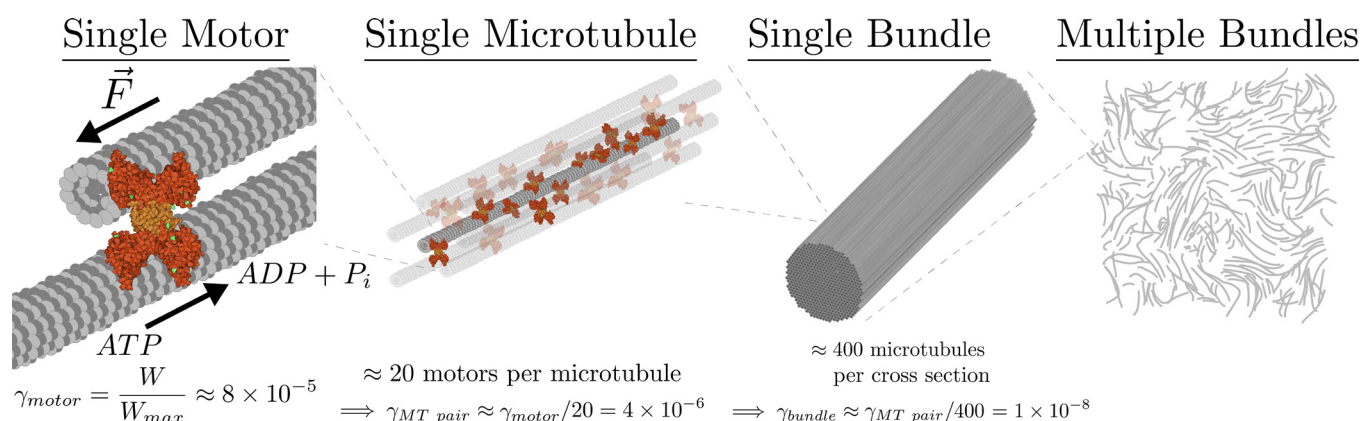
Fig. 4. Energy propagation across scales. Inefficiencies in the conversion of energy into motion happen at a number of scales. At the motor scale, moving a microtubule through water requires far less energy than is released through ATP hydrolysis. At the microtubule scale, many motors cross-linking a microtubule cause the microtubule to move at most at the speed of a single motor, but each motor hydrolyzes ATP. At the bundle scale, many microtubules are in a cross-section, but as the aspect ratio of bundles is large, fluid motion is approximately independent of bundle diameter. At the system scale, the interaction between multiple bundles could lead to further energetic losses.
