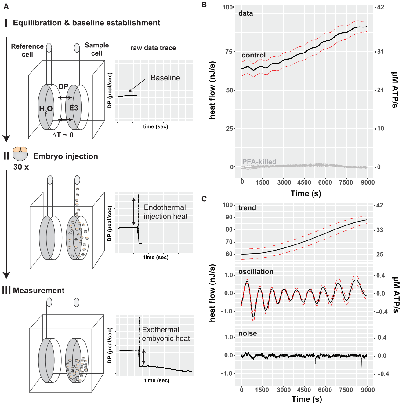
Figure 1. Isothermal Calorimetry of Synchronized Cleavage Stage Embryos Reveals Oscillatory Heat Flow Atop an Increasing Trend
